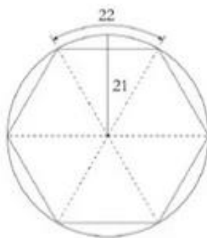
The Geometry of \pi as 22/7
