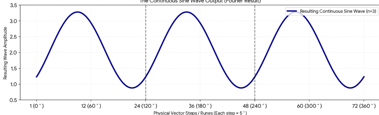
The Continuous Sine Wave Output (Fourier Result)
